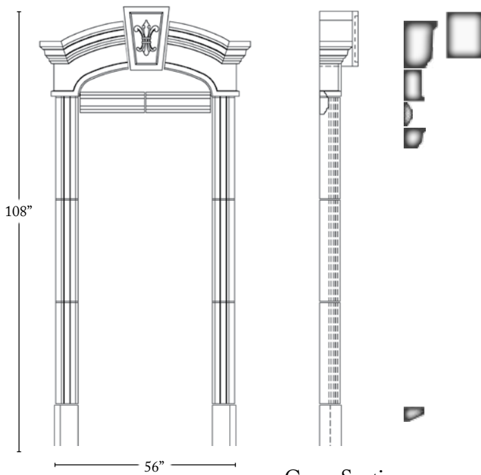
Cross Section
